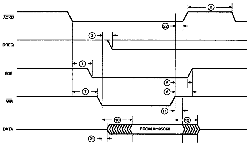
DMA Fly-By Read Cycle
