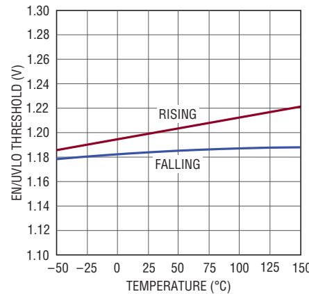
EN/UVLO Threshold Voltage
