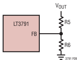
Figure 9. Resistor Connection for Open LED Protection
