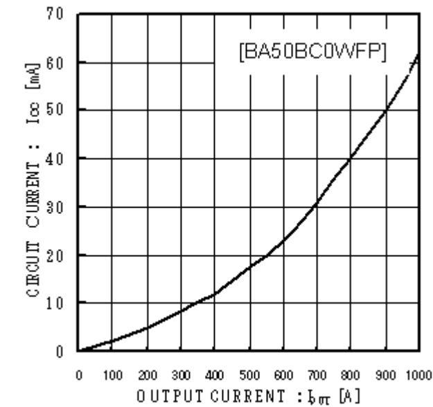
Fig.12 Circuit Current Classified by Load
