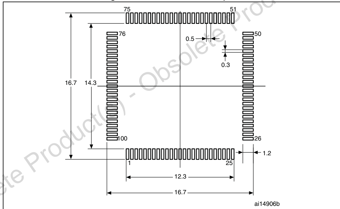
Figure 32. Recommended footprint
