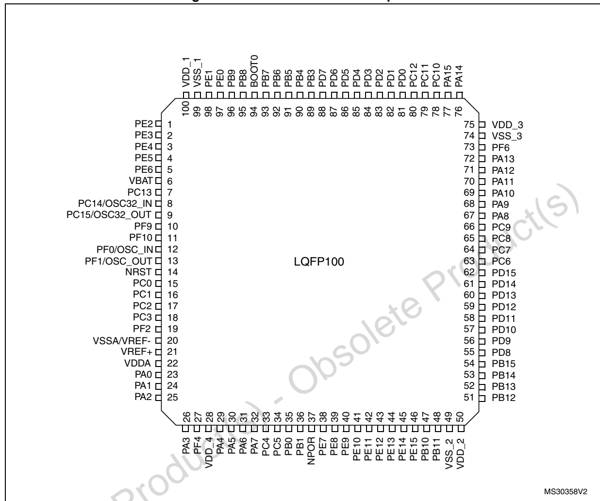
Figure 6. STM32F313xx LQFP100 pinout
