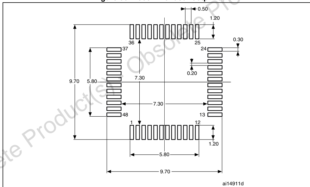
Figure 36. Recommended footprint
