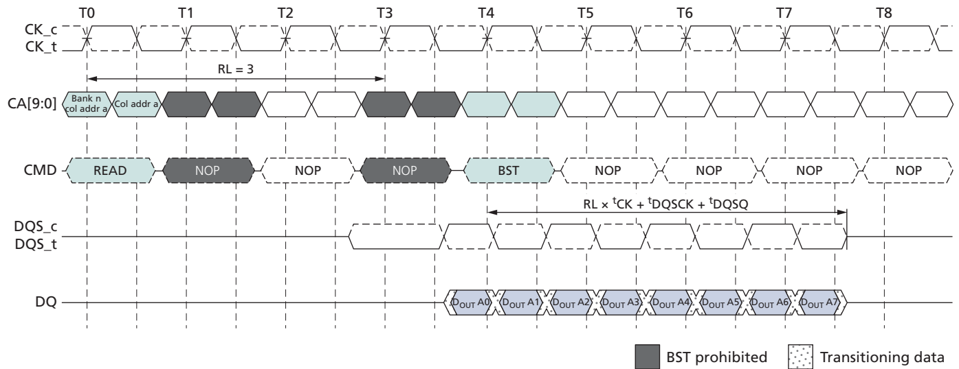
Figure 33: Burst READ Truncated by BST – RL = 3, BL = 16
