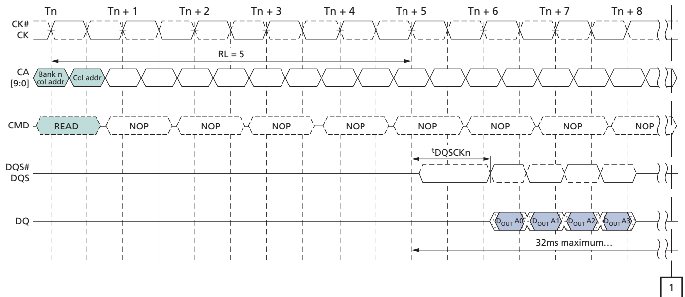
Figure 21: t_{DQSKDL} Timing
