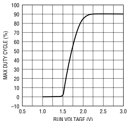
Max % DC vs RUN/SS Voltage
