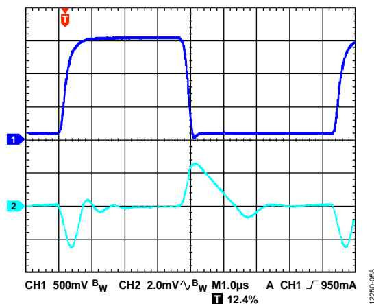
Figure 58. Output Transient Response, V_{OUT} = 5\text{ V} , C_{OUT} = 4.7\text{ }\mu\text{F}
