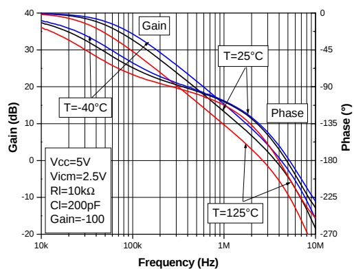
Figure 11. Voltage gain and phase with C_L = 200 pF
