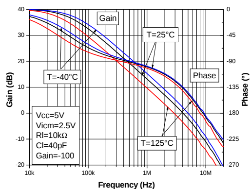
Figure 9. Voltage gain and phase with C_L = 40 pF
