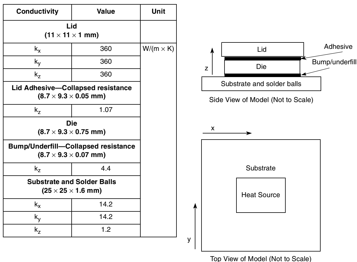
Figure 44. MPC8555E Thermal Model
