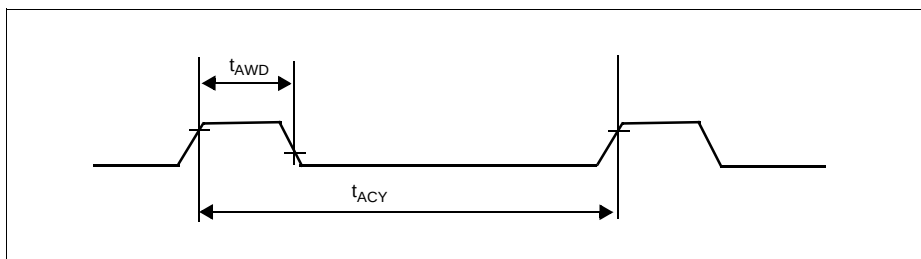
Figure 31 ALE Characteristic
