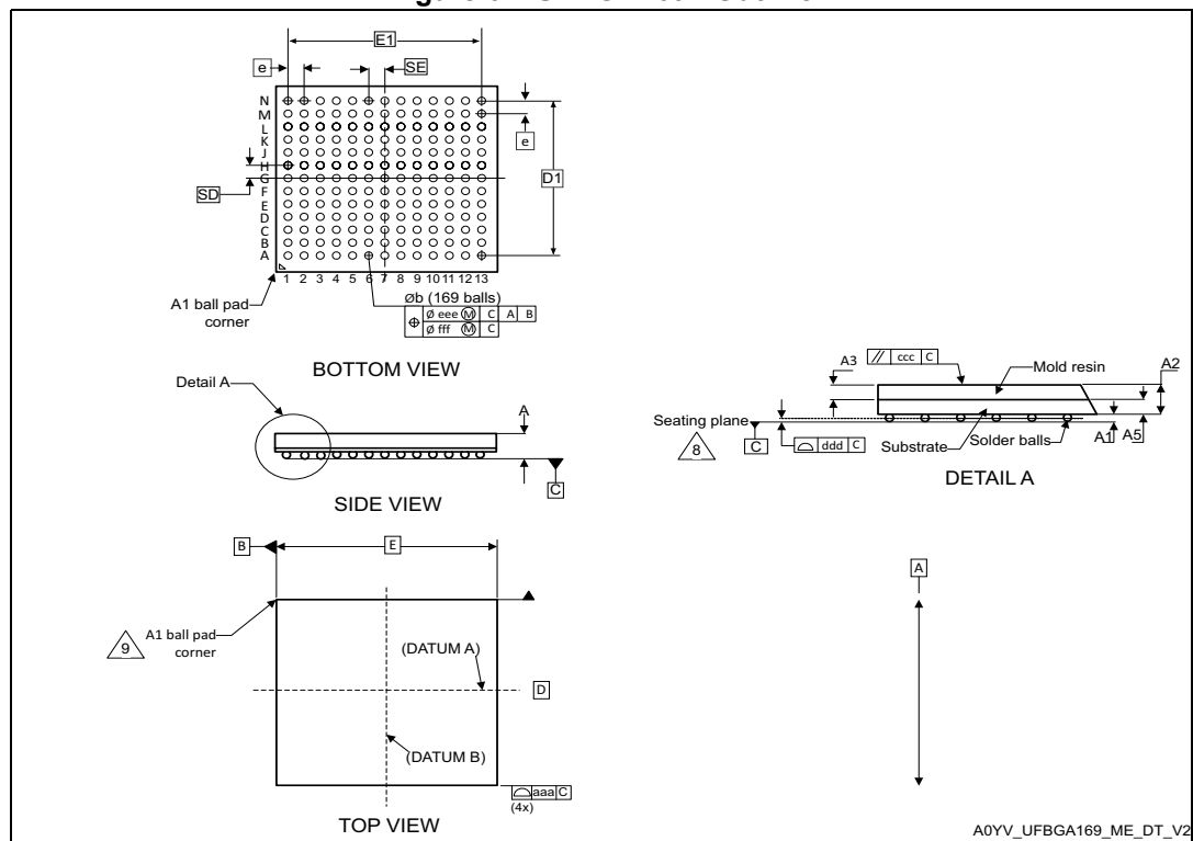
Figure 64. UFBGA169 - Outline
