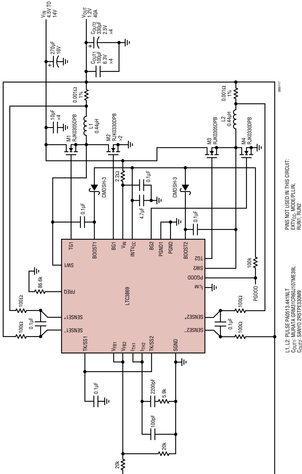
Figure 17. High Efficiency Dual Phase 1.2V, 40A Supply, f_{sw} = 250kHz
