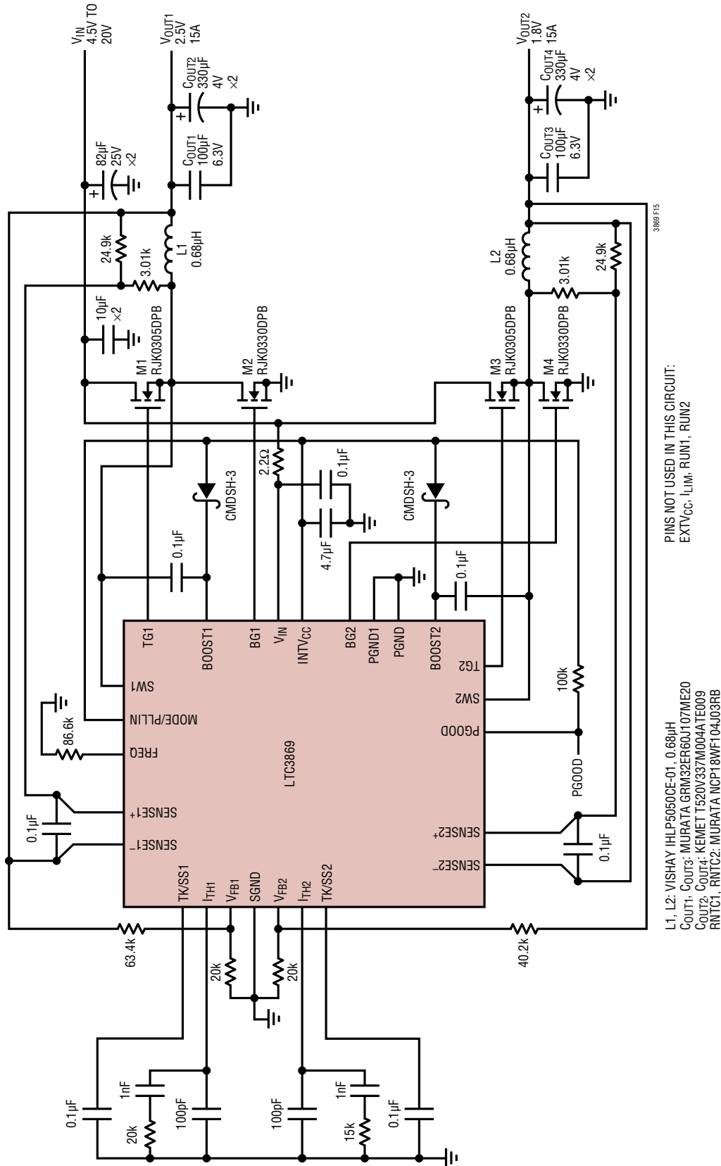
Figure 15. 2.5V, 15A and 1.8V, 15A Supply with DCR Sensing, f_{sw} = 350kHz
