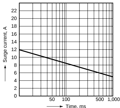
2-2. Surge current and time (IDC)
