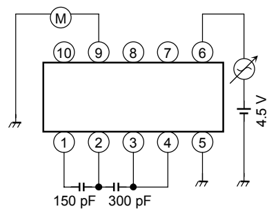
(b) DIFF-AMP PSRR
