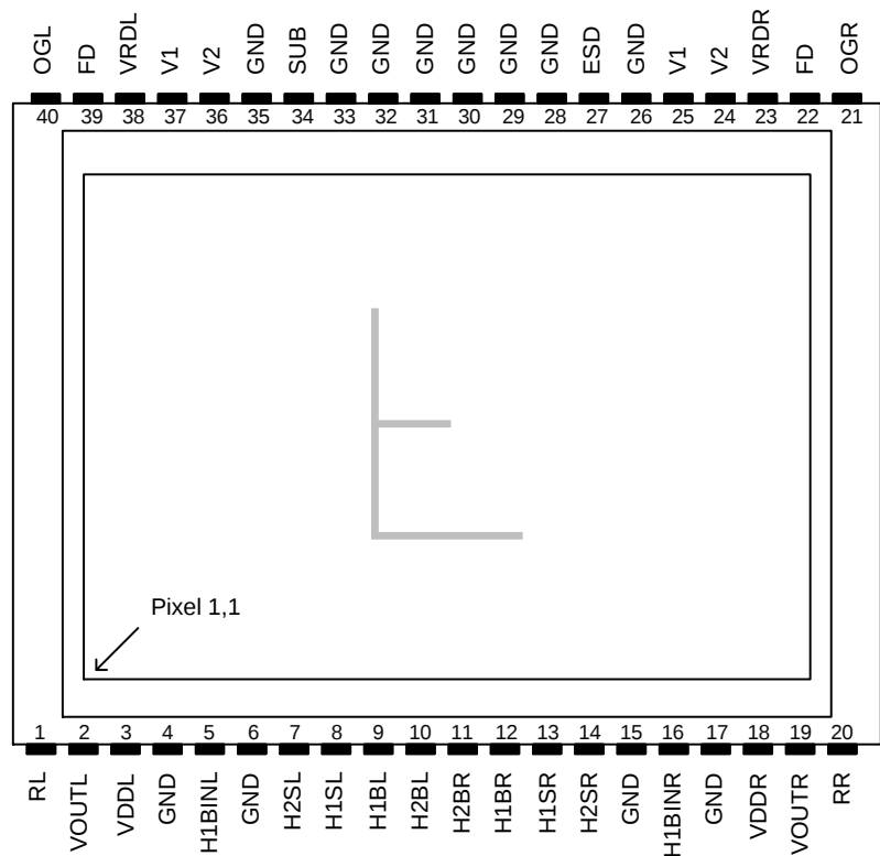
Figure 8. Pin Description
