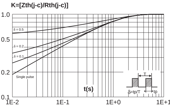
Fig. 11: Relative variation of thermal impedance junction to case versus pulse duration
