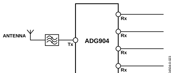
Figure 28. Tx/Rx Switching
