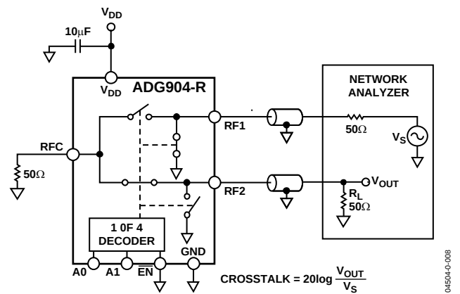
Figure 22. Crosstalk
