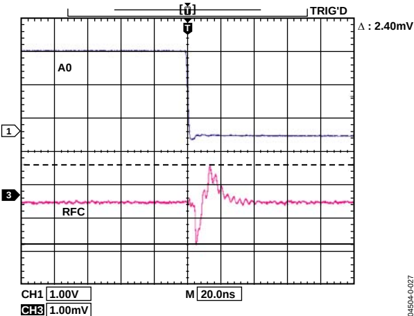
Figure 15. Video Feedthrough
