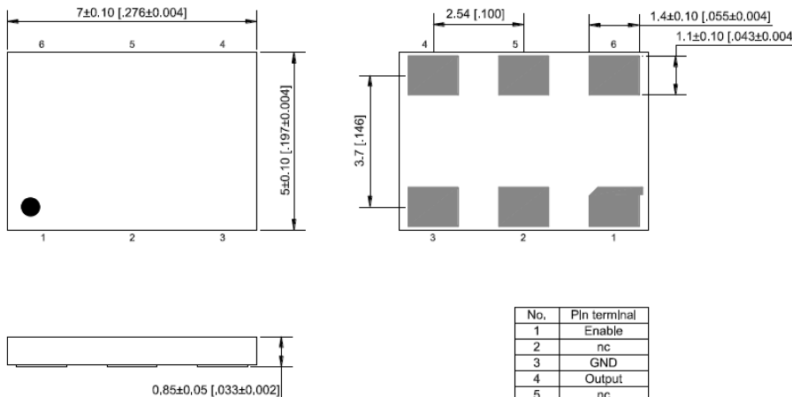
External Dimensions
