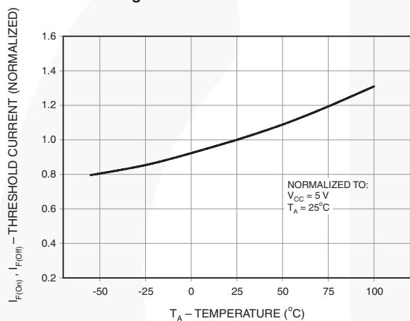
Figure 5. Threshold Current vs. Supply Temperature
