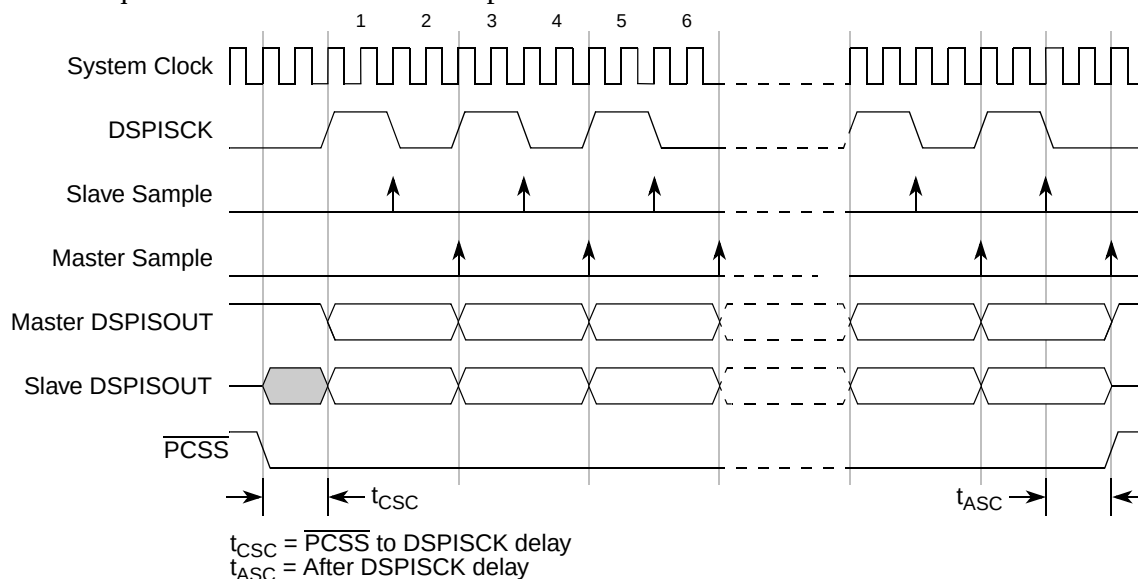
Figure 28-18. DSPI Modified Transfer Format (MTFE = 1, CPHA = 1, Fscck = Fsys/4)
