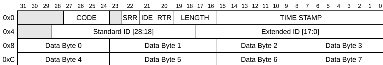
Figure 21-12. Message Buffer Structure for Both Extended and Standard Frames
