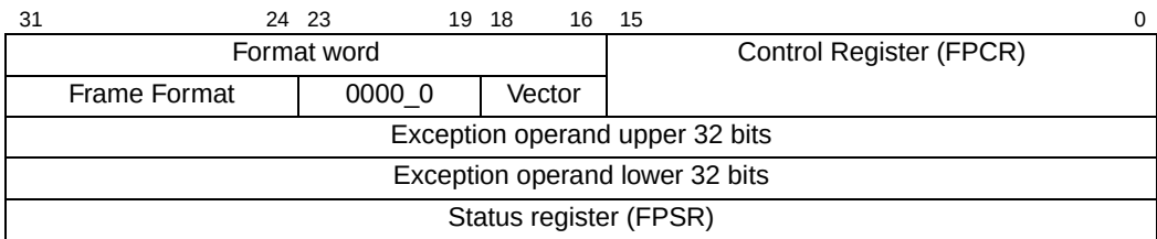
Figure 6-13. Floating-Point State Frame Contents
