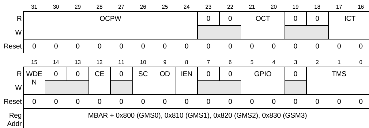
Figure 11-1. GPT Enable and Mode Select Register (GMSn)
