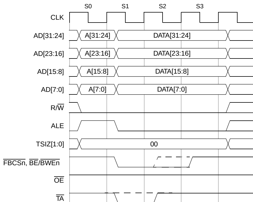
Figure 17-17. Longword Write Transfer with Muxed 32-A / 32-D
