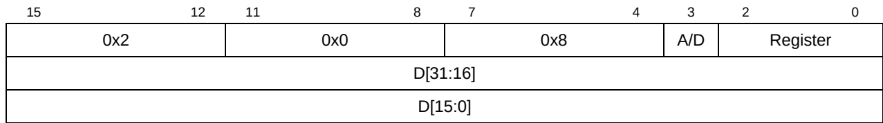
Figure 8-25. WAREG/WDREG Command Format
