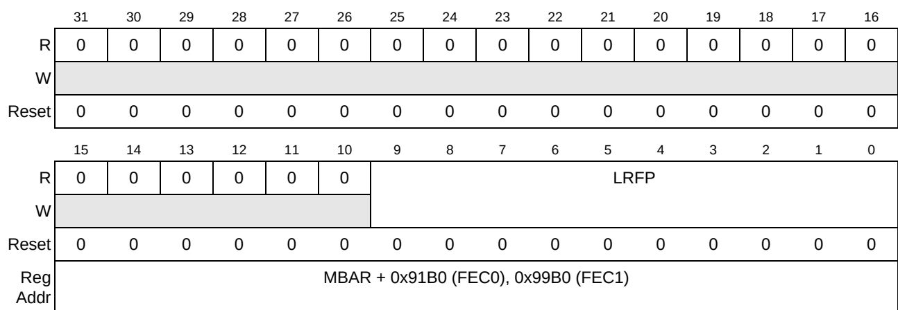
Figure 31-32. FEC Transmit FIFO Last Write Frame Pointer Register (FECTLWFP)
