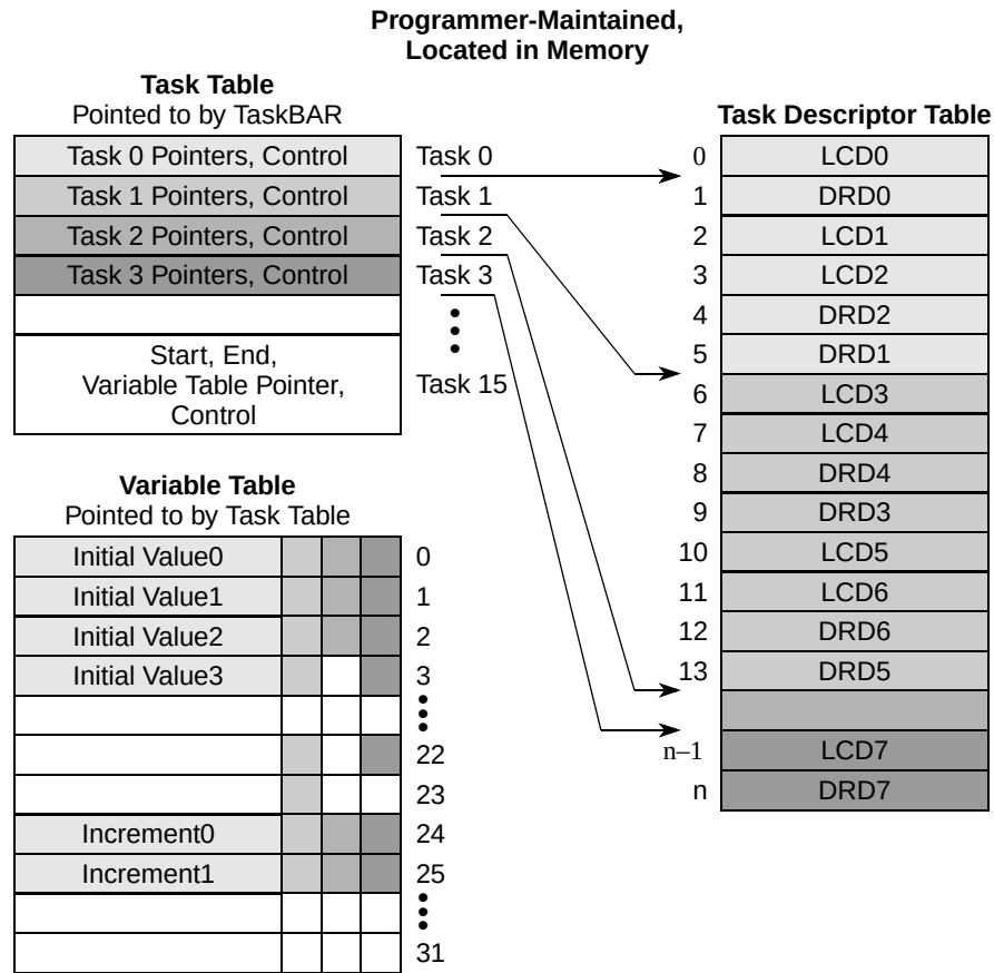
Figure 24-2. DMA Programmer-Maintained Memory Model
