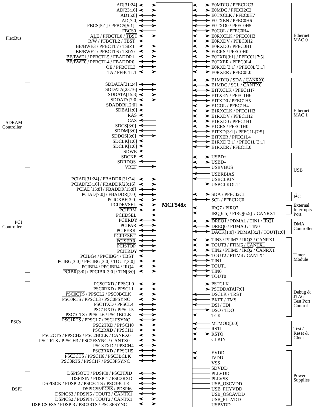
Figure 2-1. MCF548x Signals
