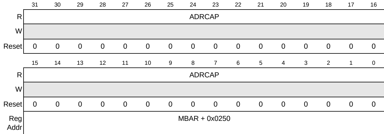
Figure 10-9. Arbiter Address Capture Register (XARB_ADRCAP)
