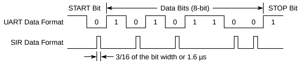
Figure 27-44. Data Format in SIR Mode
