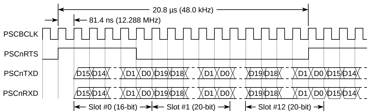
Figure 27-41. Waveform of AC97 Mode
