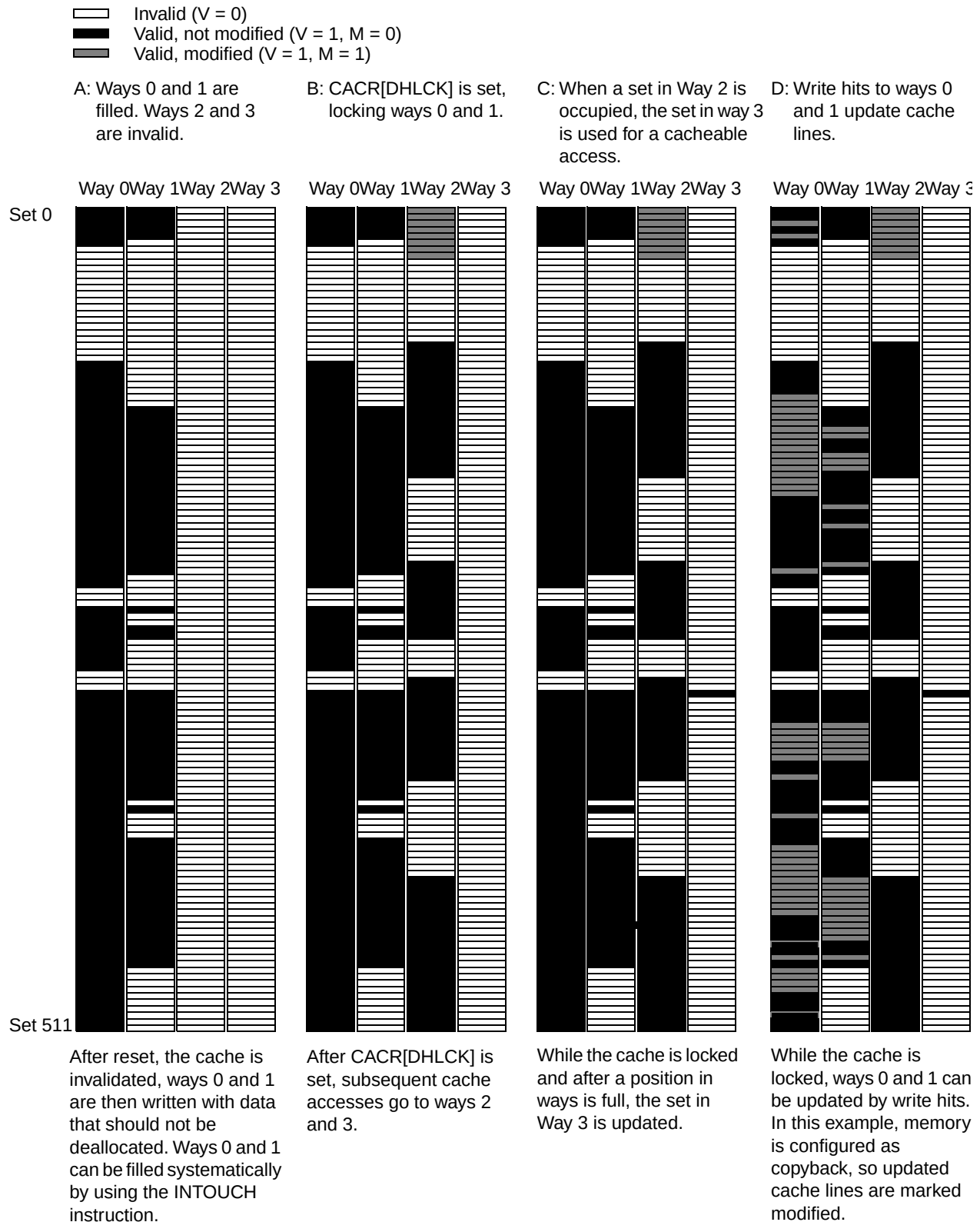
Figure 7-7. Data Cache Locking
