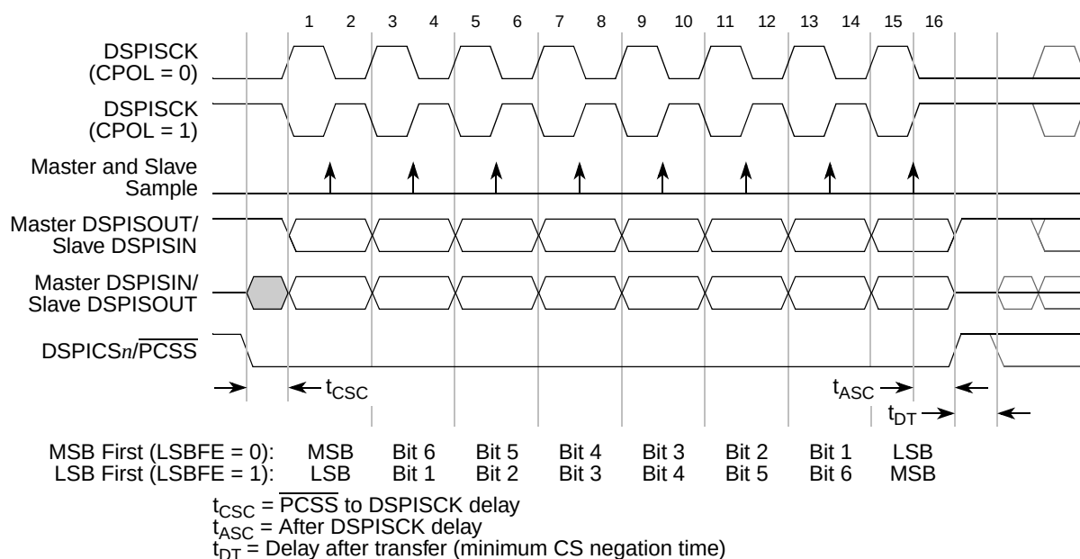
Figure 28-16. DSPI Transfer Timing Diagram (MTFE = 0, CPHA = 1, FMSZ = 8)
