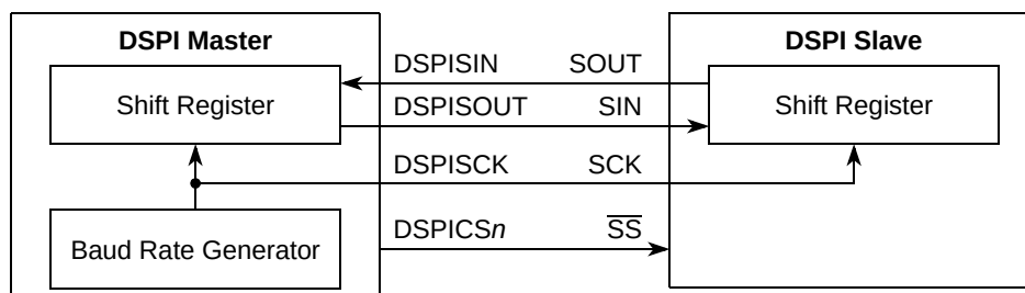
Figure 28-11. SPI Serial Protocol Overview
