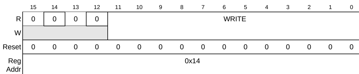
Figure 25-7. Write Pointer Register
