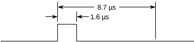
Figure 27-47. Serial Interaction Pulse (SIP)
