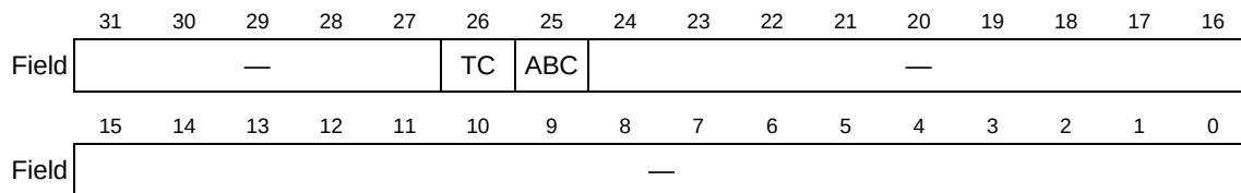
Figure 31-40. Transmit Frame Control Word Format (TFCW)
