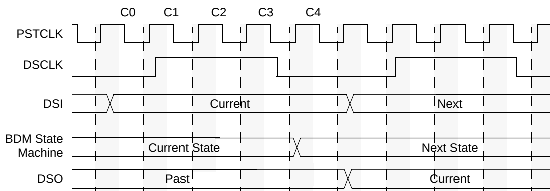
Figure 8-18. Maximum BDM Serial Interface Timing
