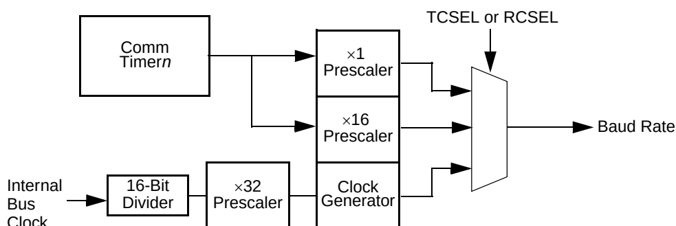
Figure 27-5. UART and SIR Baud Rate Clocking Sources
