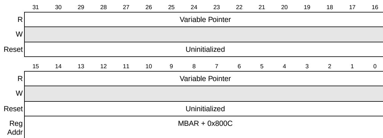
Figure 24-6. Variable Pointer Register (VP)
