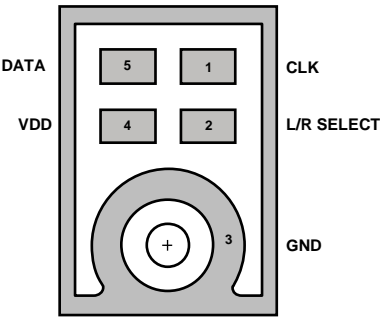
Figure 3. Pin Configuration
