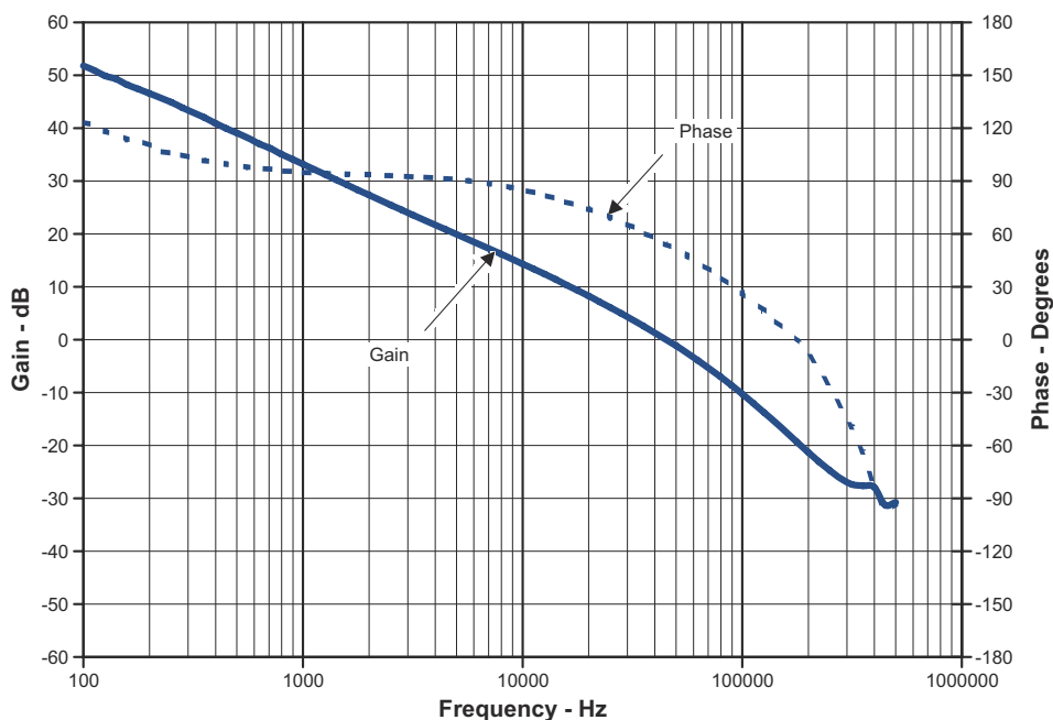
Figure 2-6. TPS54623EVM-012 Loop Response
