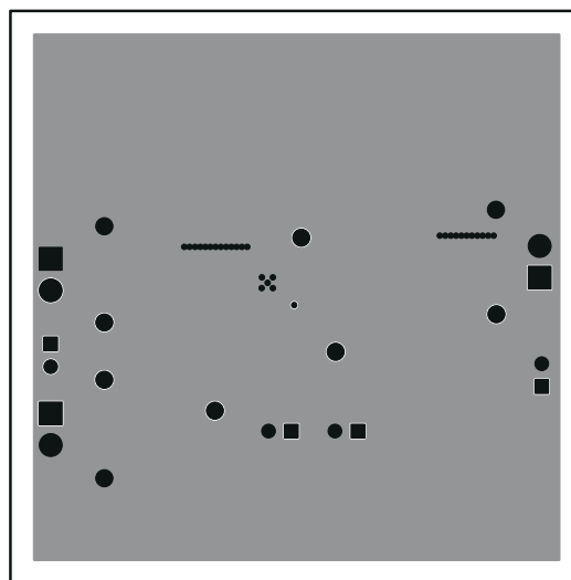
Figure 3-2. TPS54623EVM-012 Layout 2
