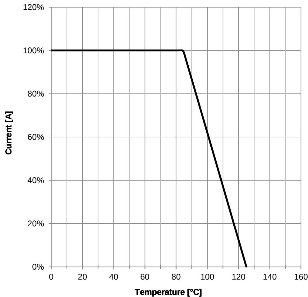
Derating Curve:
