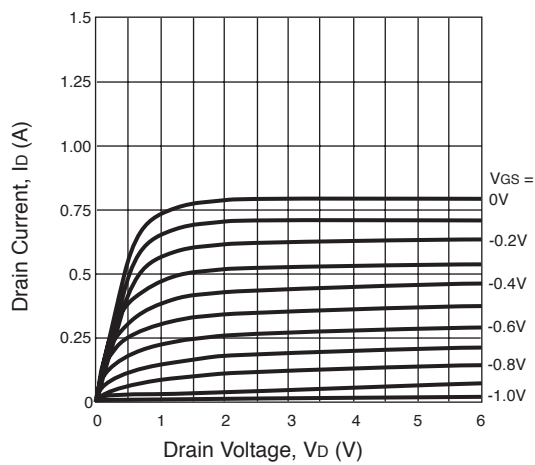
DRAIN CURRENT vs. DRAIN VOLTAGE
