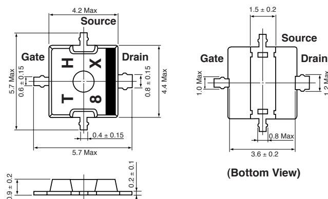
PACKAGE OUTLINE 79A
