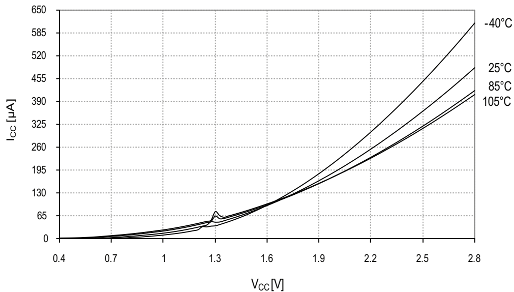
Figure 33-143. Power-on reset current consumption vs. V_{CC} .
