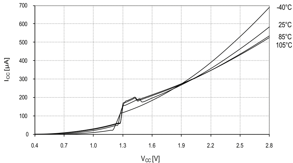
Figure 33-143. Power-on reset current consumption vs. V_{CC} .
