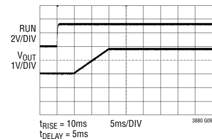
Soft-Start Ramp
