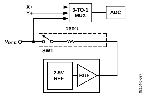
Figure 27. On-Chip Reference Circuitry
