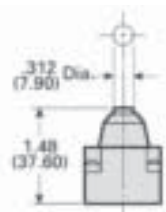
Plain top plunger
