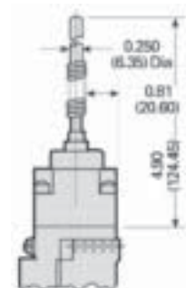
Wobble head with nylon head 3SE03-DW1 3SX03-KW2
