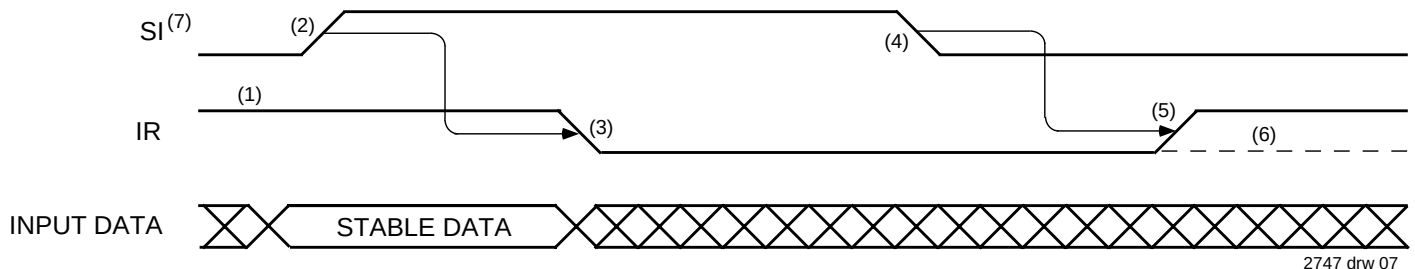
Figure 2. Input Timing
