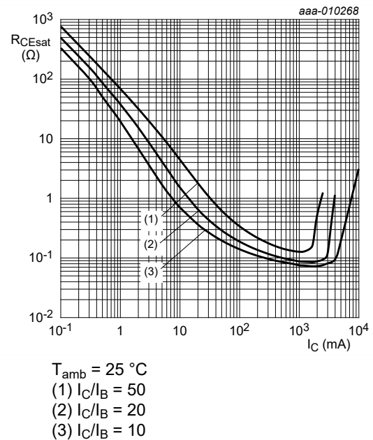
Fig. 11. TR1 (NPN): Collector-emitter saturation resistance as a function of collector current; typical values
