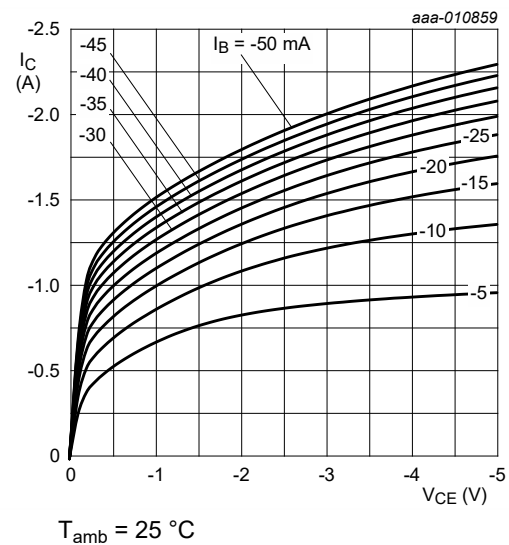
Fig. 13. TR2 (PNP): Collector current as a function of collector-emitter voltage; typical values
