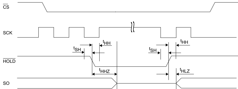
Figure 22. \overline{\text{HOLD}} Timing
