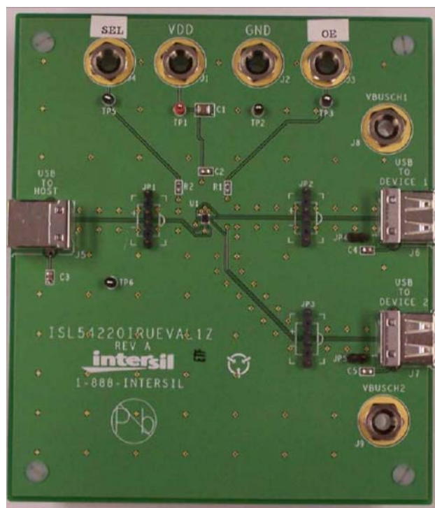
FIGURE 1. ISL54220IRUEVAL1Z EVALUATION BOARD
