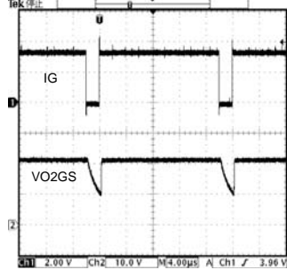
Fig. 24 Gate Shading Output Waveform
