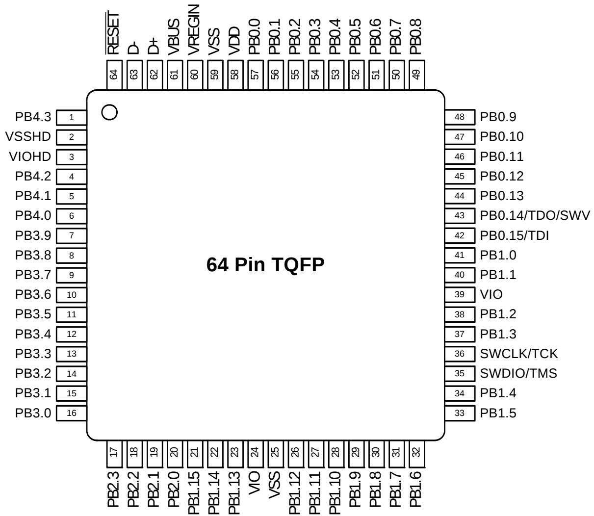
Figure 5.3. SiM3U1x6-GQ Pinout
