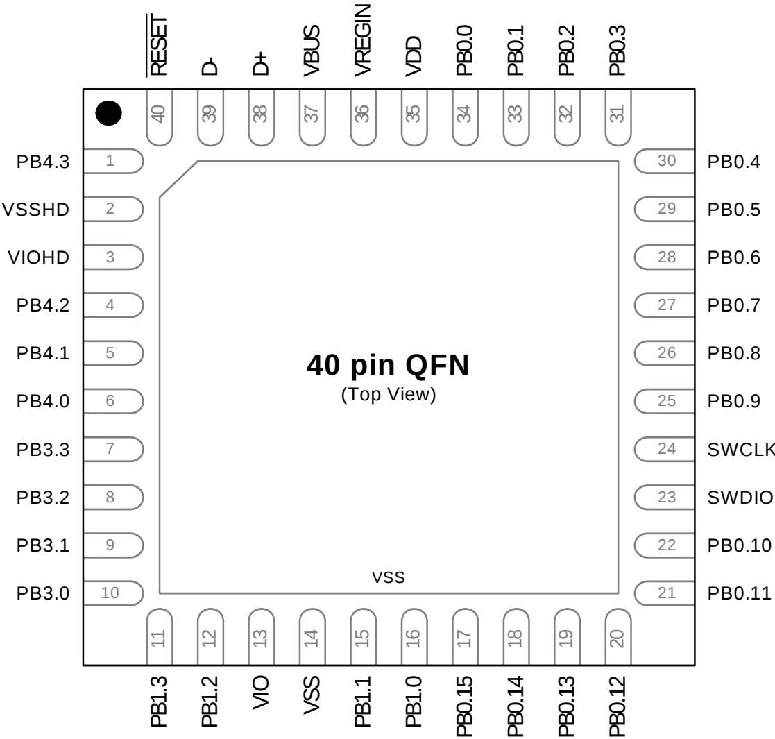
Figure 5.5. SiM3U1x4-GM Pinout
