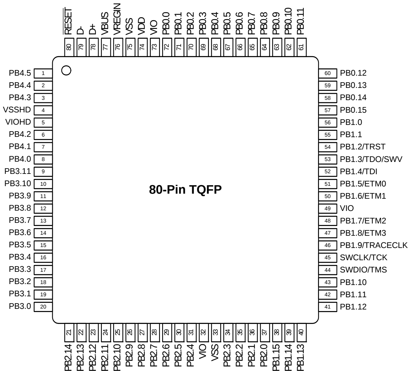
Figure 5.1. SiM3U1x7-GQ Pinout
