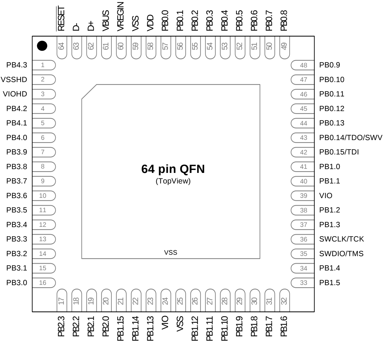
Figure 5.4. SiM3U1x6-GM Pinout
