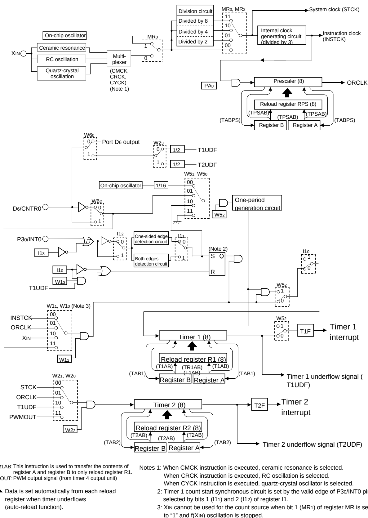
Fig. 25 Timer structure (1)
