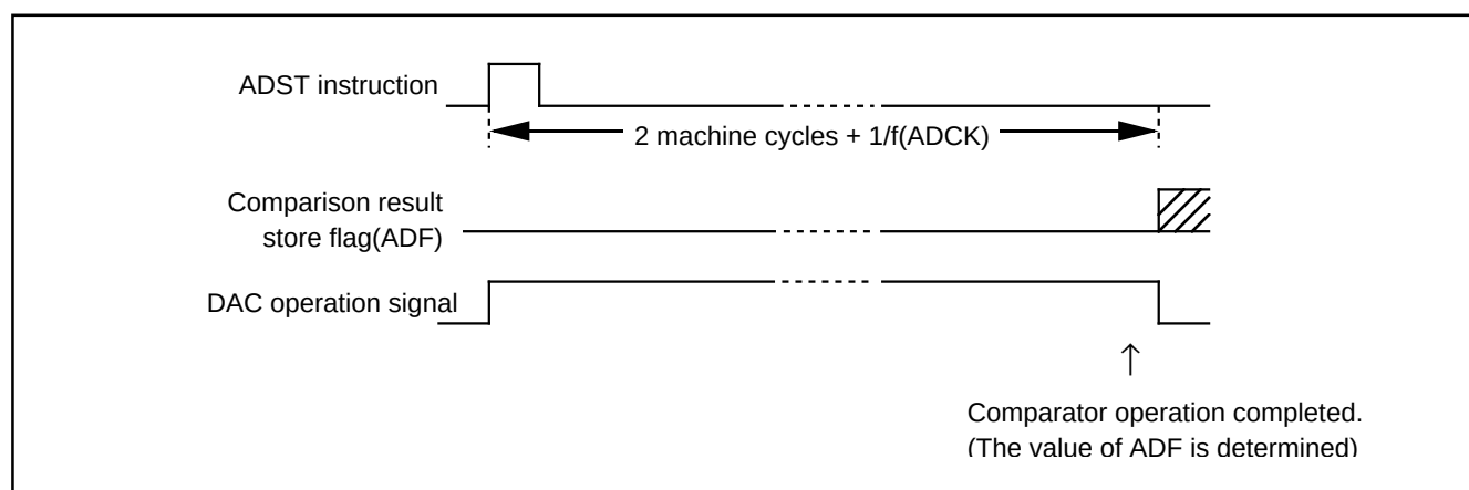
Fig. 40 Comparator operation timing chart
