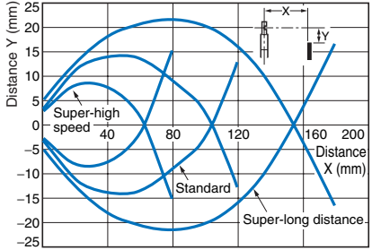
Reflective E32-D61
