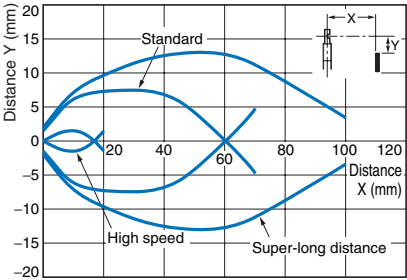
Reflective E32-D36P1
