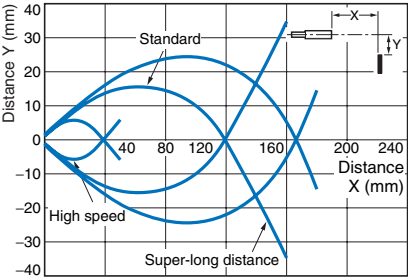
Reflective E32-D24R
