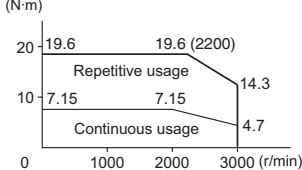
R88M-G1K520T (1.5 kW)
