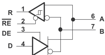
Figure 10-3. Logic Diagram
