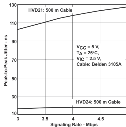
Figure 8-8. SN65HVD2[1,4] Peak-to-Peak Jitter vs Signaling Rate
