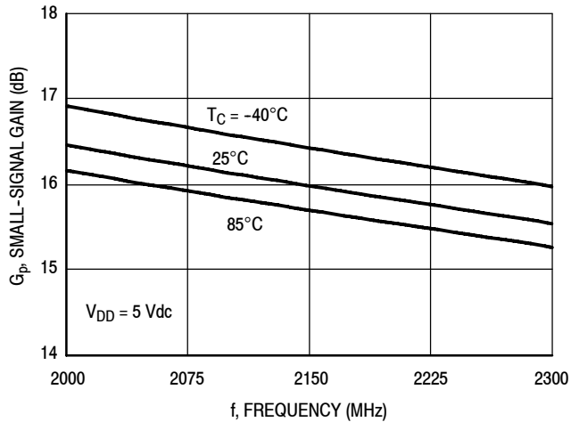
Figure 4. Small-Signal Gain (S21) versus Frequency
