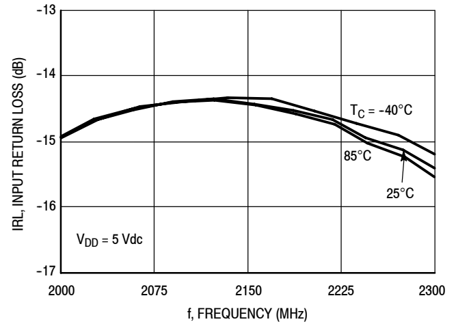
Figure 5. Input Return Loss (S11) versus Frequency
