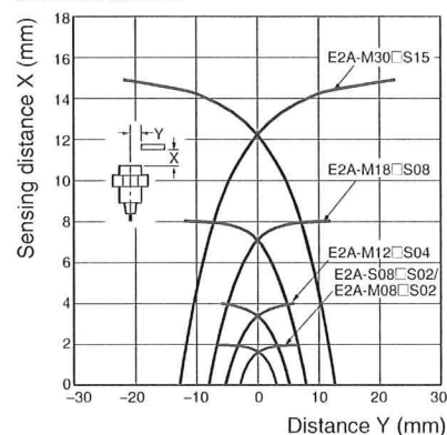
Shielded Models
