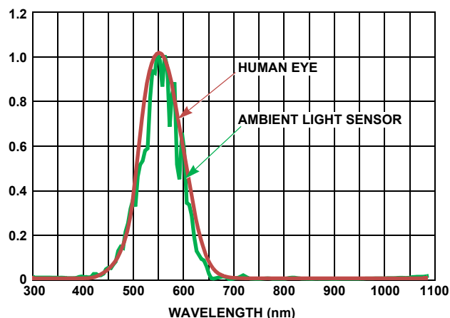
FIGURE 6. NORMALIZED SPECTRAL RESPONSE FOR AMBIENT LIGHT SENSING
