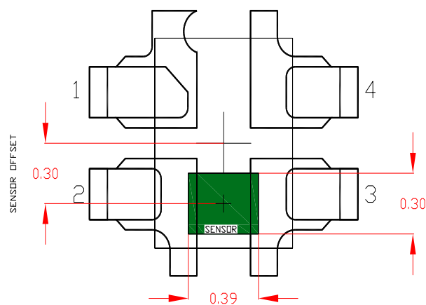
FIGURE 17. 4 LD ODFN SENSOR LOCATION OUTLINE
