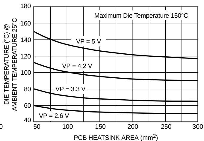
Figure 32. Maximum Die Temperature vs. PCB Heatsink Area
