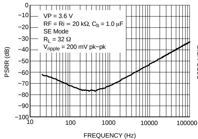
Figure 18. PSRR (SE Mode) @ VP = 3.6 V
