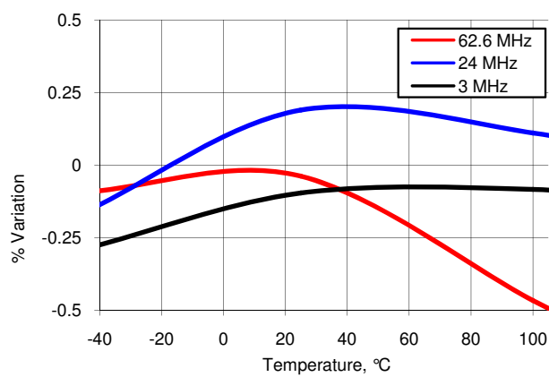
Figure 11-3. IMO Frequency Variation vs. Temperature
