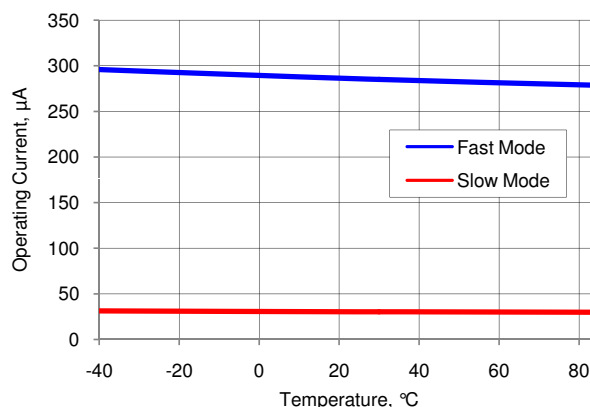
Figure 11-10.IDAC Operating Current vs Temperature, Range = 255 \mu A, Code = 0, Sink Mode
