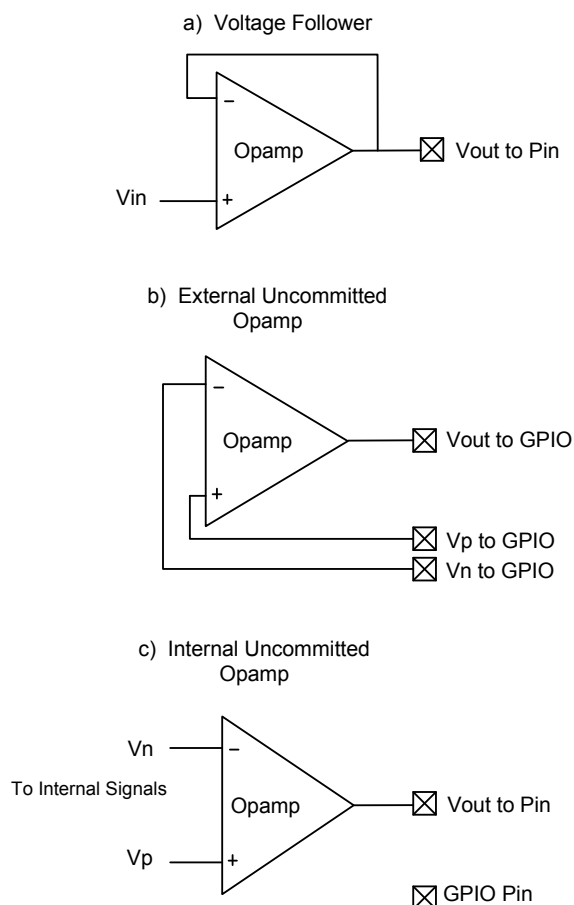
Figure 8-4.Opamp Configurations
