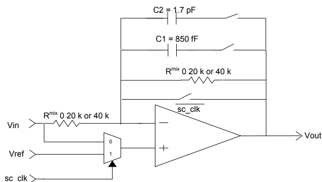
Figure 8-1.Mixer Configuration
