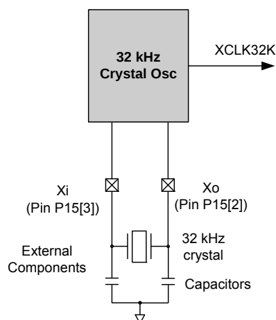
Figure 6-4.32kHzECO Block Diagram
