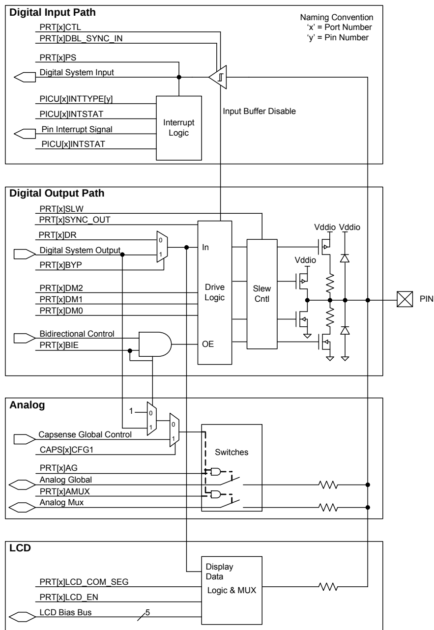
Figure 6-3.GPIO Block Diagram
