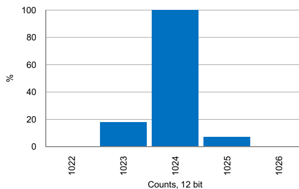
Figure 11-14.SAR ADC Noise Histogram, 1 msp, Internal Reference Bypassed
