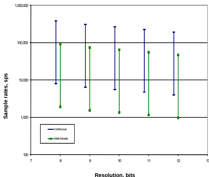
Figure 8-2. Delta-sigma ADC Sample Rates, Range = \pm 1.024 V
