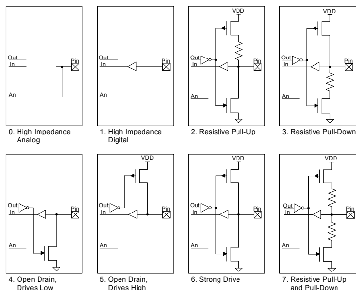
Figure 6-6. Drive Mode
