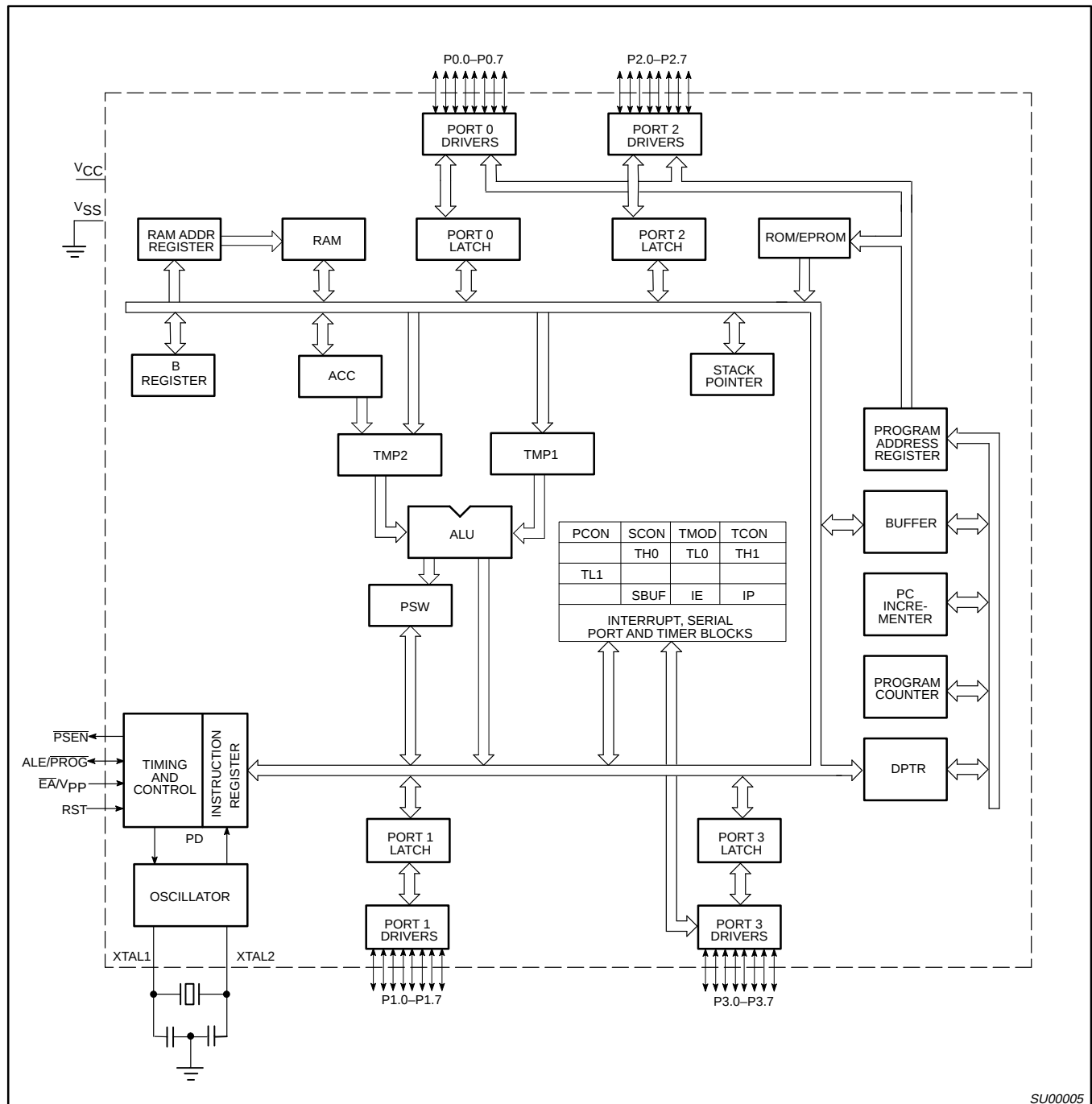
BLOCK DIAGRAM
