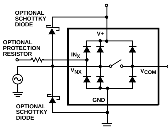
FIGURE 9. OVERVOLTAGE PROTECTION
