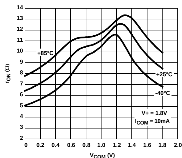
FIGURE 13. ON-RESISTANCE vs SWITCH VOLTAGE
