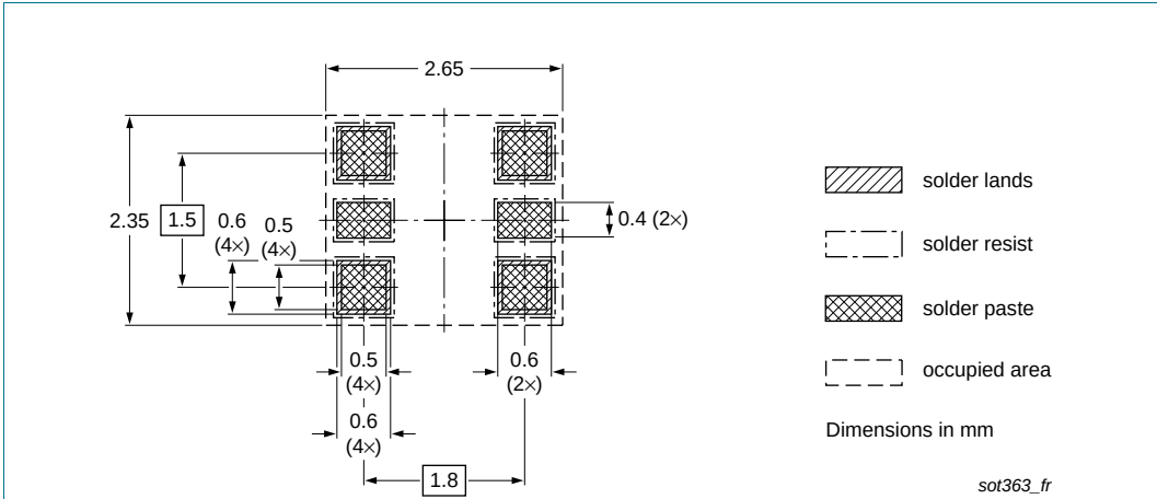
Fig 15. Reflow soldering footprint BAV756S and BAW56S (SOT363/SC-88)
