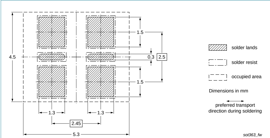
Fig 15. Reflow soldering footprint BAV756S and BAW56S (SOT363/SC-88)
