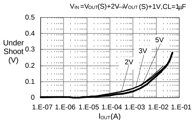
V_{DD} dependencies of undershoot at power fluctuation
