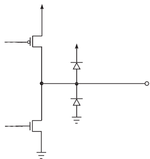
Figure 3-8: Indicator Outputs: SD/H \overline{D} , LD
