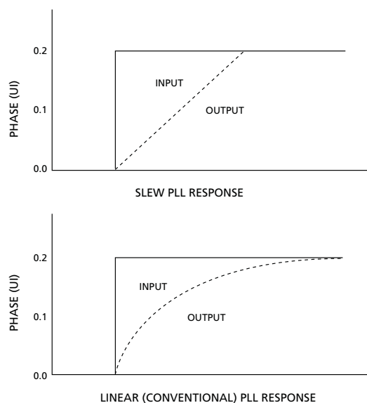
Figure 4-1: PLL Characteristics
