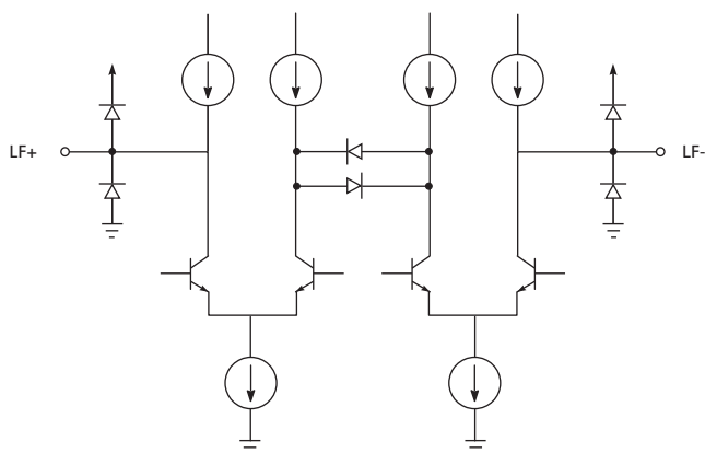
Figure 3-3: Loop Filter
