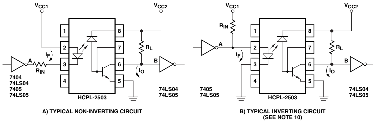
Figure 8. Recommended circuits
