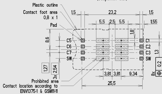
RECOMMENDED PC BOARD LAYOUT (Component side)
